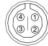
4 pins Binder 719 male connector pinout solder termination view
