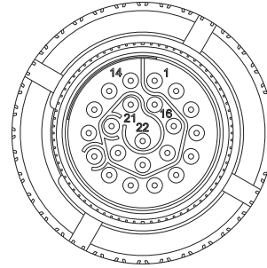
22 PINS female Deutsch connector contact insertion view
