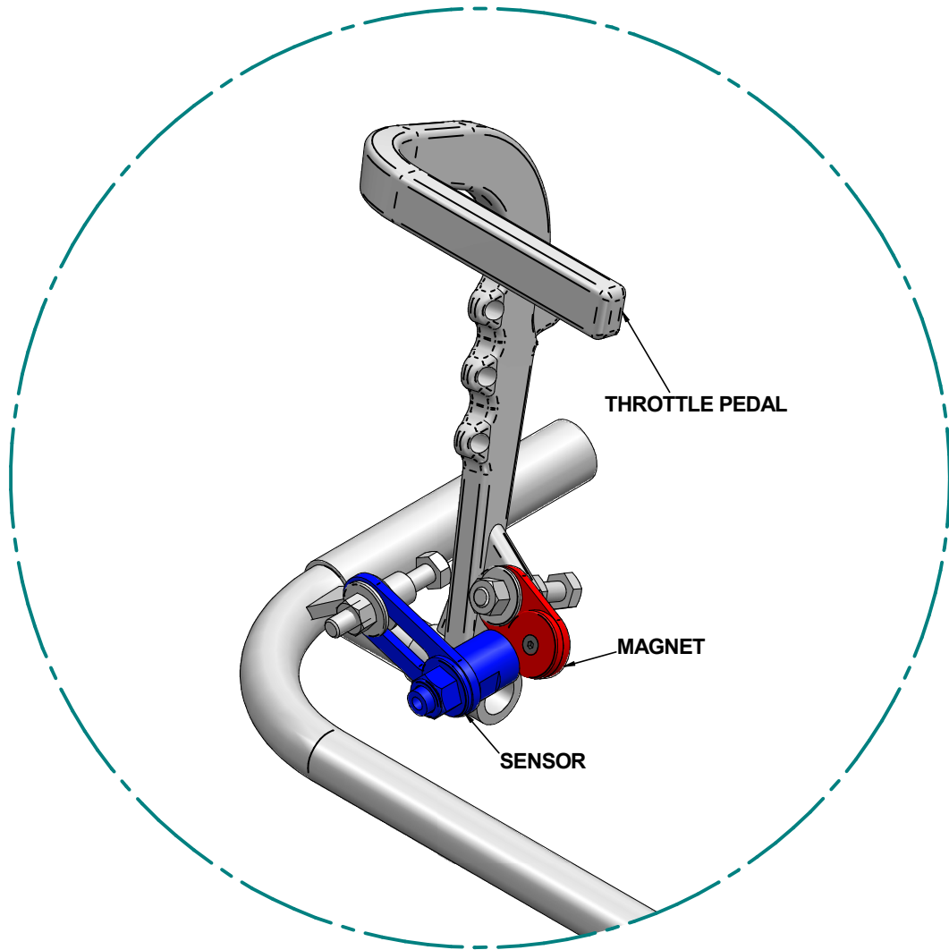
THROTTLE PEDAL SENSOR INSTALLATION EXAMPLE
