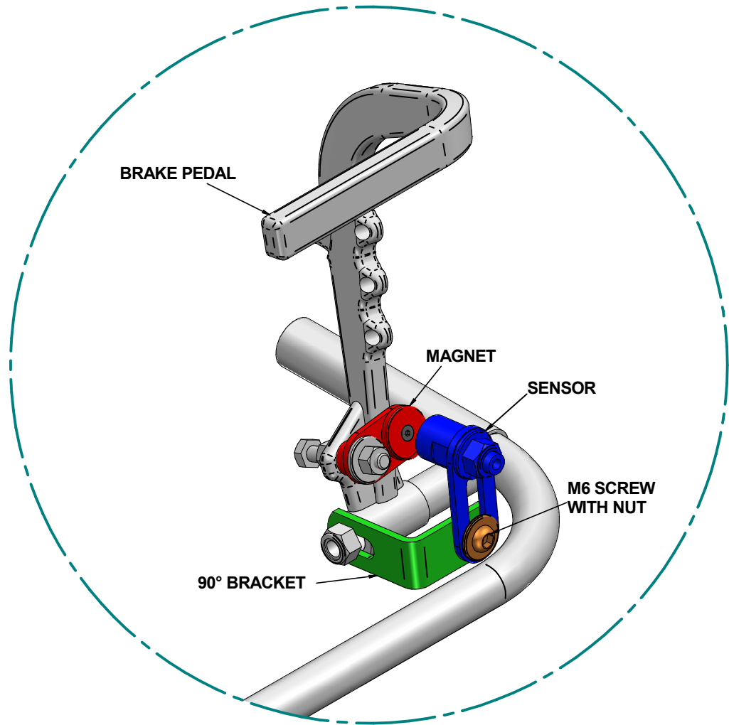
BRAKE PEDAL SENSOR INSTALLATION EXAMPLE
