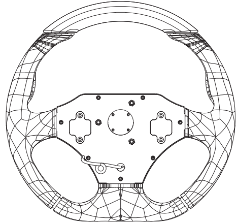
GT 350 Steering Wheel without bracket with cable X07GT350
